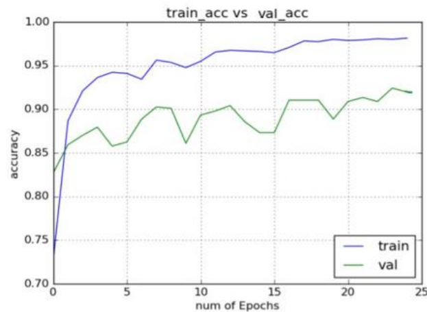
Fig 5 Accuracy graph
